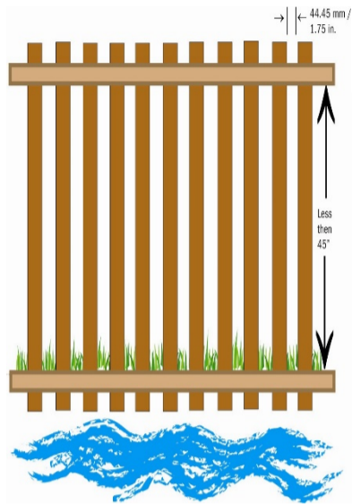
Figure 3: Vertical and horizontal member spacing and ground clearance
