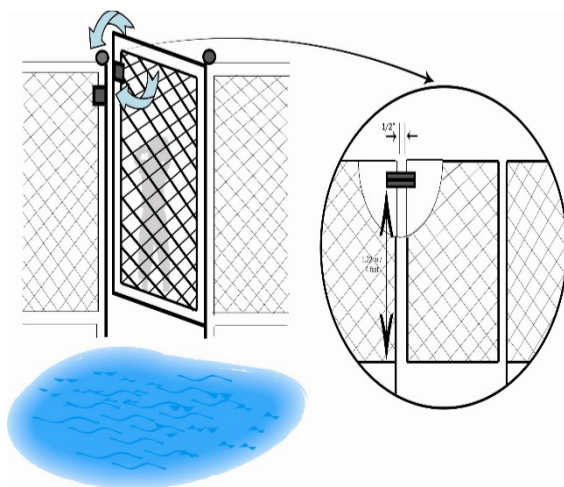
Fig. 5: Self-closing & self-latching gate installation
